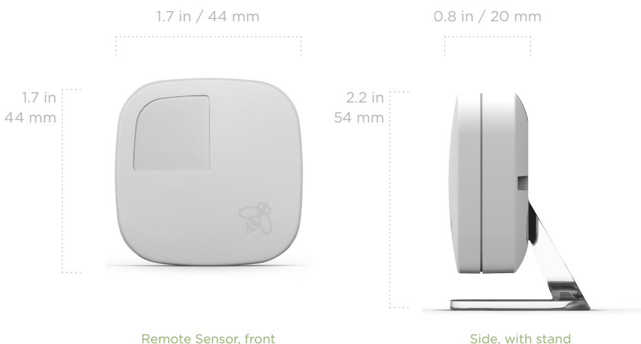
Remote Sensor, front
